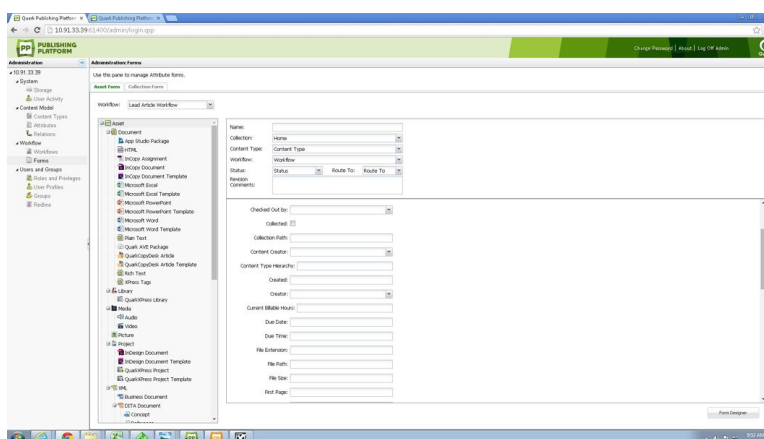
Forms pane
