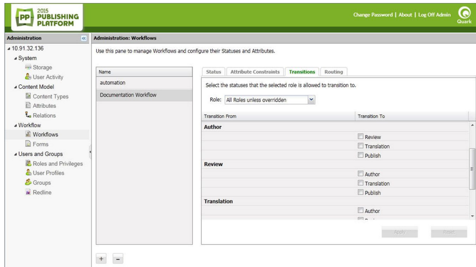
Transitions tab of the Workflows pane
