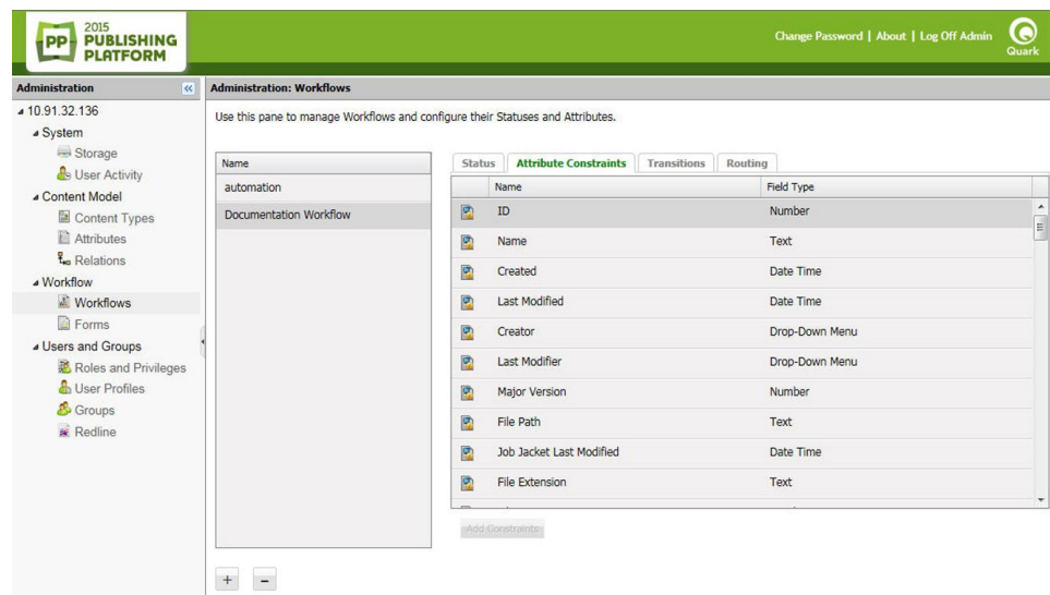
Attribute Constraints tab of the Workflows pane
